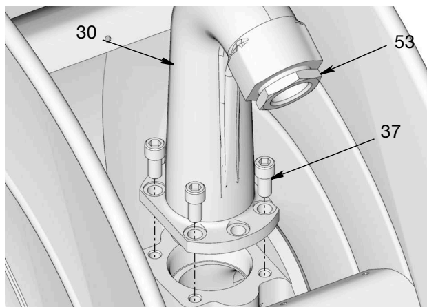
FIG. 6: Low Pressure Outlet shown. Medium Pressure models use 6 bolts.
